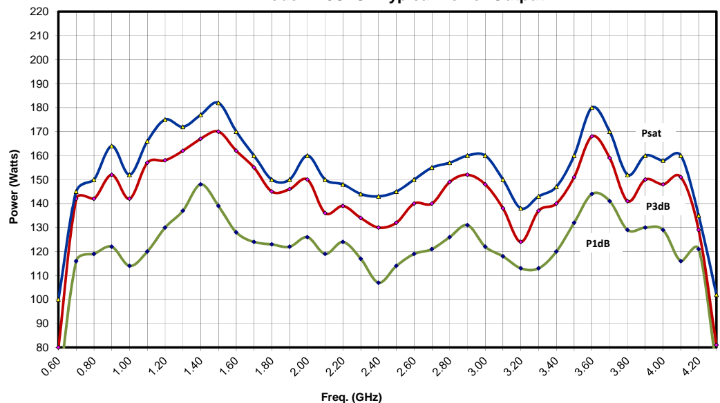
Model 125S1G4 Typical Power Output
